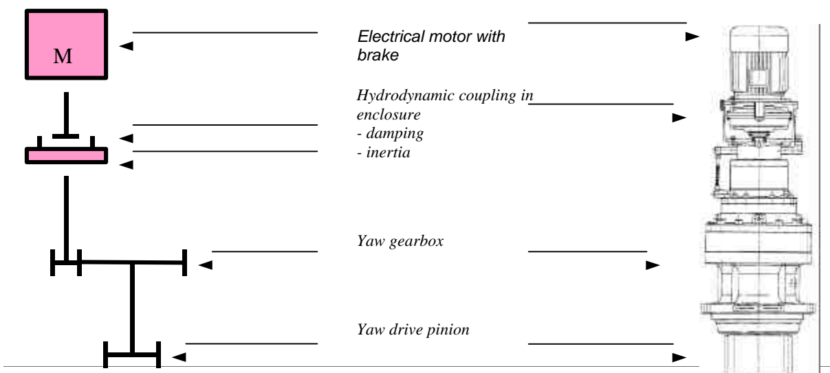
Fig. 1. Principle of a soft yaw drive.
