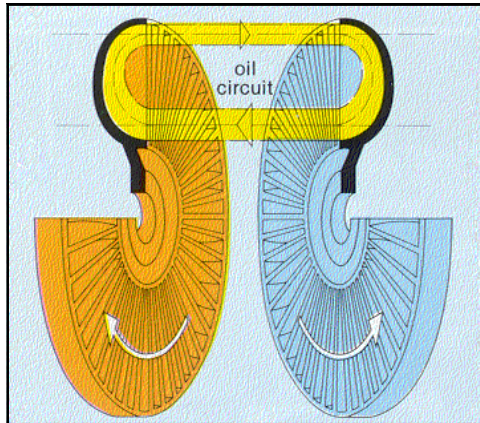
Fig. 2: Principle of hydrodynamic coupling. Sketch by courtesy of Voith.
