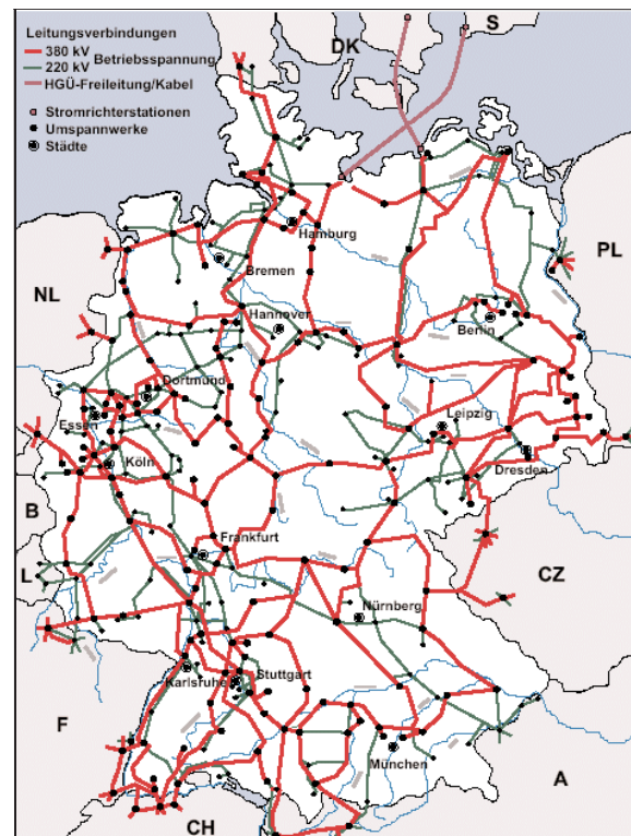
Fig. 4 High voltage distribution grid of E.on. Circles indicate the possible grid feed-in points in northern Germany [2]
