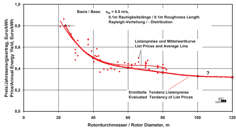
Fig. 3: Wind turbine price divided by the annual energy yield produced at the reference site which is defined in the German Renewable Energy Sources Act (EEG) [3]
