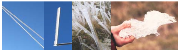
Fig. 1 Typical ice indicators: From the left, iced power lines, lightning conductor, grass on the ground, rime ice fragment from a rotor blade found on the ground.
