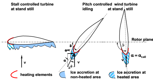
Fig. 6 Stall- and pitch-controlled wind turbine with heating elements at the leading edge during icing conditions at standstill and idling.
