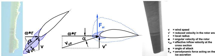
Fig. 4 Icing at leading edge at different modes of operation. Left side idling, right side power production.
