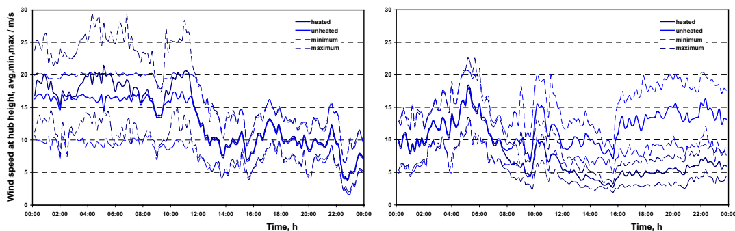
Fig. 2 Example for a two days wind speed measurement at Tauernwind. 10 - minute averages, minima and maxima of the heated and non-heated hub height anemometers.
