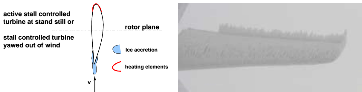
Figure 12 Stall-controlled wind turbine in icing conditions at standstill: Possible configuration if only the leading edge is heated. Observation of trailing edge icing (right side) of a stall-controlled turbine at stand still.
