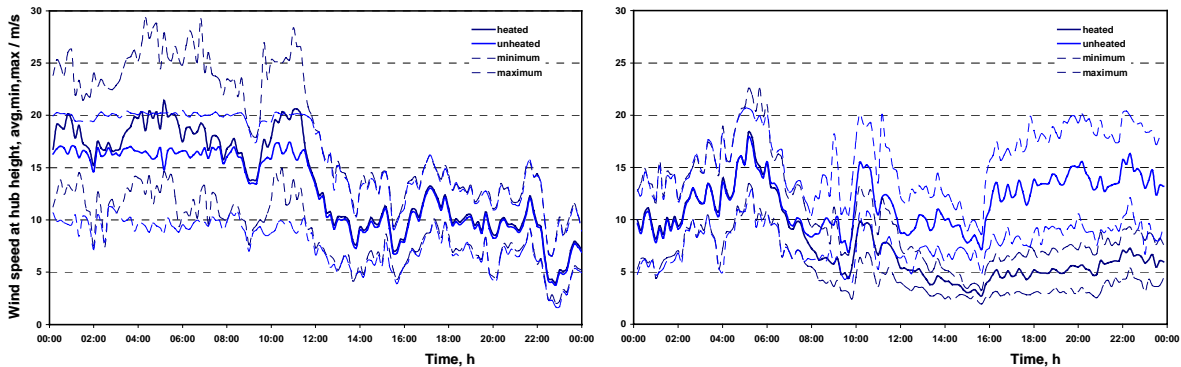
Figure 4 Example for a two days wind speed measurement at Tauernwind. 10 - minute averages, minima and maxima of the heated and non-heated hub height anemometers.
