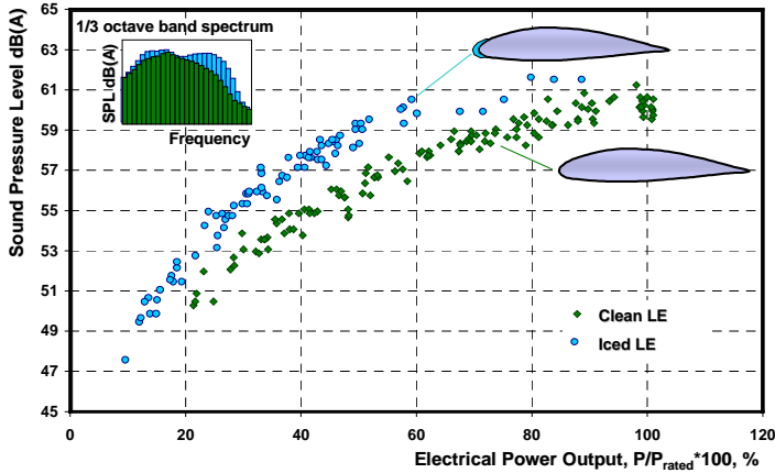
Figure 5 Acoustic noise measurement: Sound pressure level versus the normalised power output during beginning of slight icing conditions (LE = leading edge).
