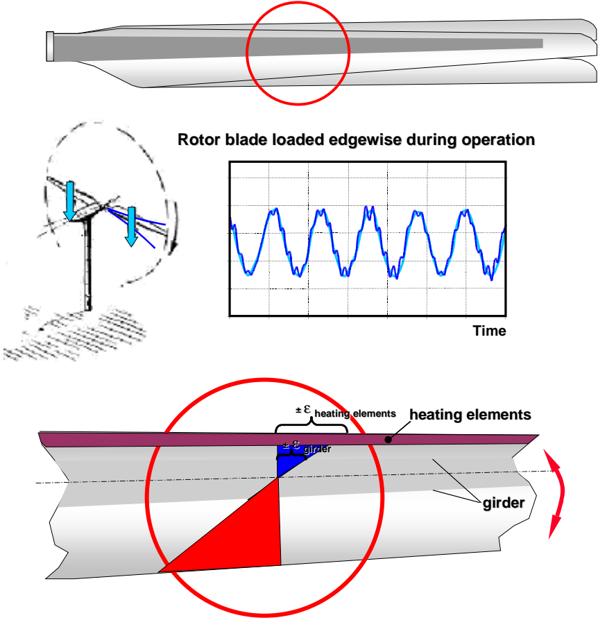
Figure 14 Loading on leading edge heating elements during operation.
