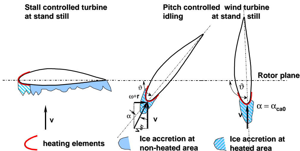
Figure 13 Stall- and pitch-controlled wind turbine with heating elements at the leading edge during icing conditions at standstill and idling.
