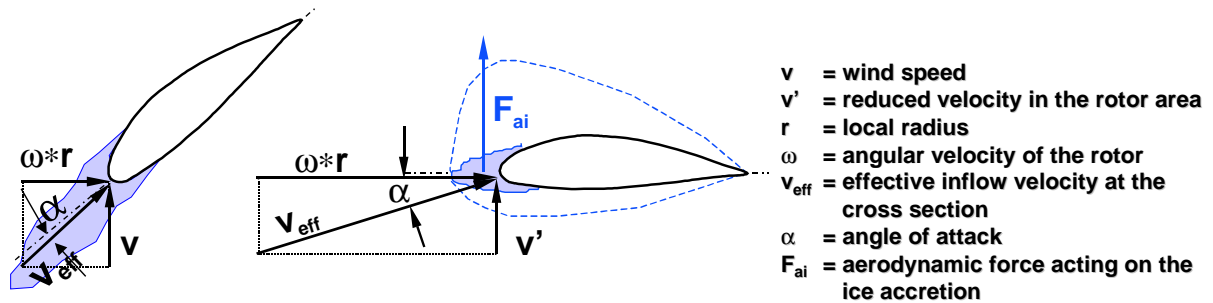
Figure 7 Icing at leading edge at different modes of operation. Left side idling, right side power production.
