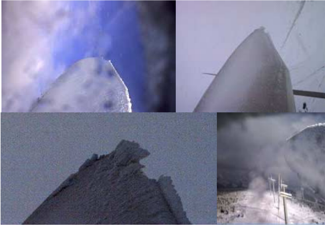
Figure 15 Pictures taken by WEB camera from the hub of one of the Tauernwind turbines
