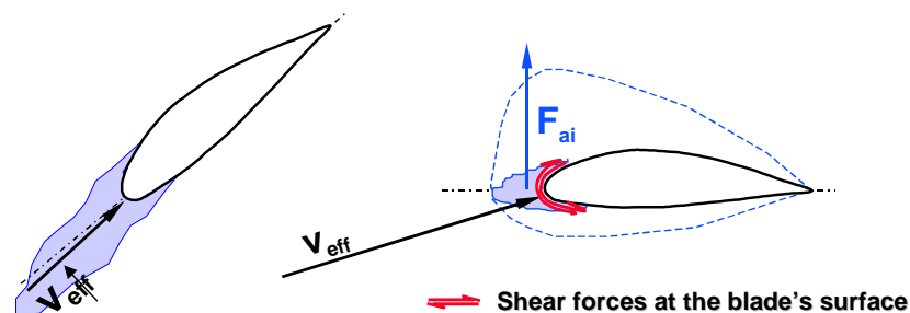
Figure 9 Shear forces between ice accretion and blade's surface during idling and operation (right side).
