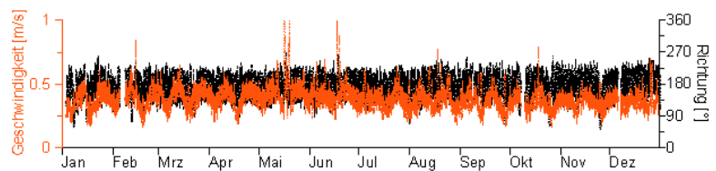
Fig. 3: 2005 current statistics at 8 m depth level at FINO 1. The main direction is on the 260 - 80° axis, and the current speed is mostly between 0.4 and 0.65 m/s. The time series below shows the average over a tide cycle.
