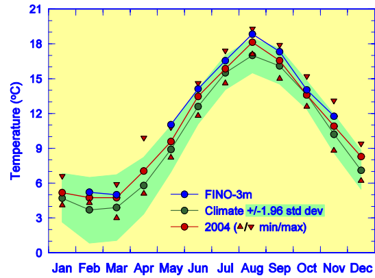
Fig. 2: Temperature data measured at 3 m depth at the FINO 1 platform in 2004 (blue dots) in comparison with the data from "Helgoland Reede" as monthly averages of the years 1970 to 2000 (green dots), the double standard deviation (light green band) and the monthly average of 2004
