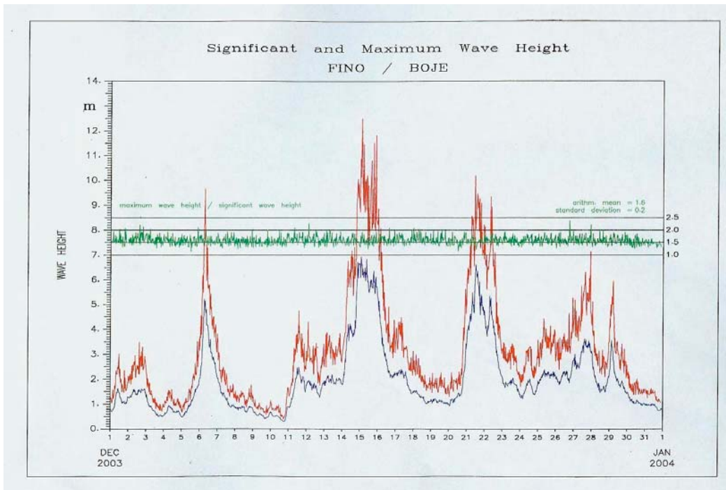
Fig. 4: December 2003, significant wave heights ( H_s , blue line), measured maximum wave heights ( H_{max} , red line) and the relation H_{max}/H_s with an average of 1.6.
