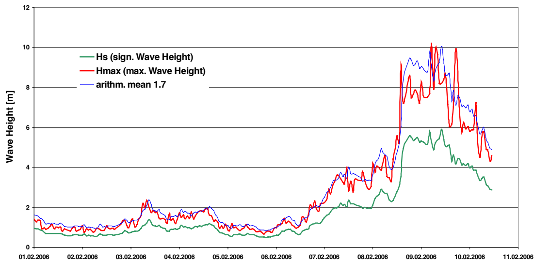
Fig. 5: FINO1 - Storm event on 9 February 2006. The time series shows the significant wave heights (green line), measured maximum wave heights (red line), and the calculated maximum wave heights (blue line, H_s multiplied by the arithmetic mean of 1.7).
