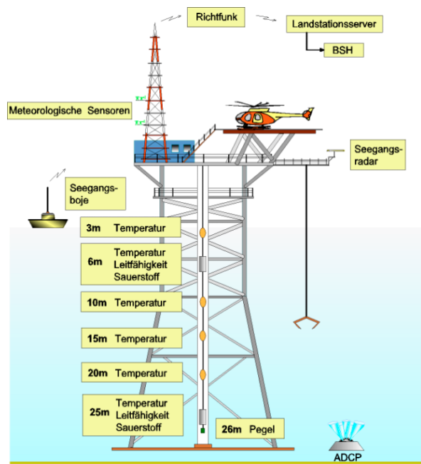
Fig. 1: Measuring concept for oceanographic variables at FINO 1, which includes data on sea state, currents, temperatures, conductivity, pressure, and oxygen.
