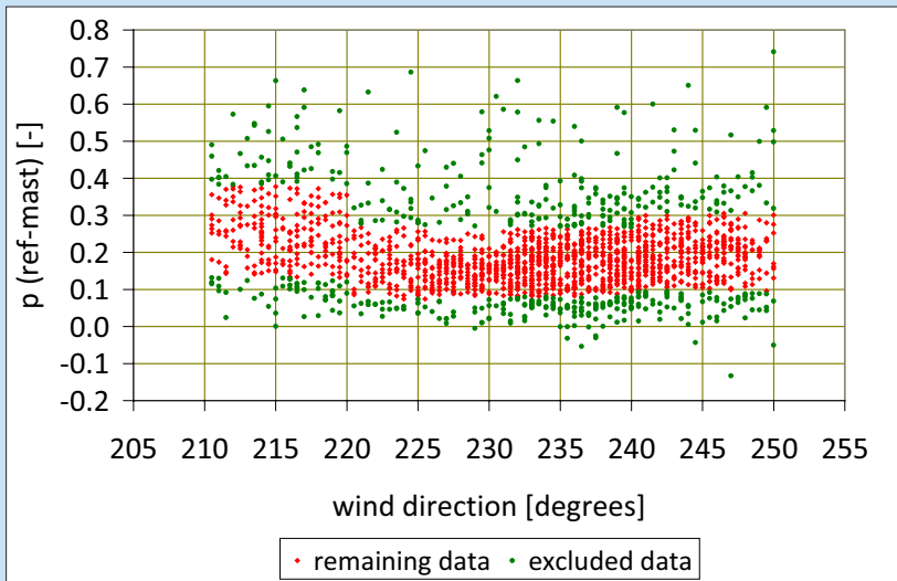
Fig. 3: Wind shear exponent p at ref-mast for main data base and filtered data set after applying the wind profile filter (sc 5) for expected later measurement sector, wind speed range: ]4 m/s ; 16 m/s], temperature > 2°C.
