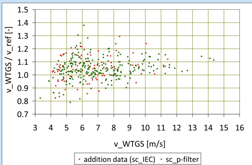
Fig. 4: Site calibration correction factor versus wind speed measured at WTGS-mast for the different data bases (sc 1), wind speed range: ]4 m/s ; 16 m/s], temperature > 2°C, one 5 degrees sector with maximum slope of 14.6 degrees within 4D from ref-mast.
