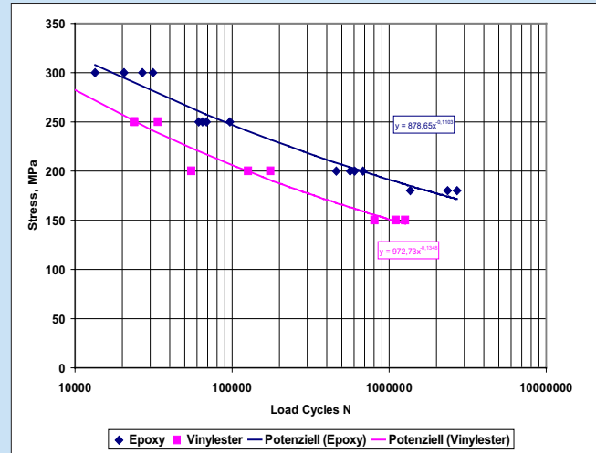
Fig. 2: S-N curves of Triax/UD-laminates, Hexion-measurement
