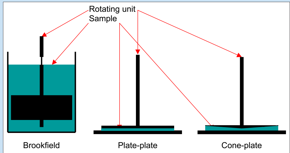
Fig. 3: Different rotating viscometer types for measuring the rheological behaviour
