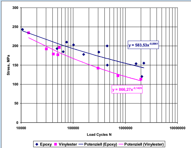
Fig. 1: S-N curves of Triax/UD-laminates, Risø-measurement
