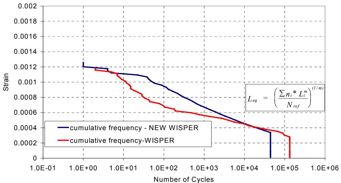
Fig.6: WISPER and NEW WISPER Cumulative Range Pair Spectra – Calibrated for Equal Strain at Max Load Level
