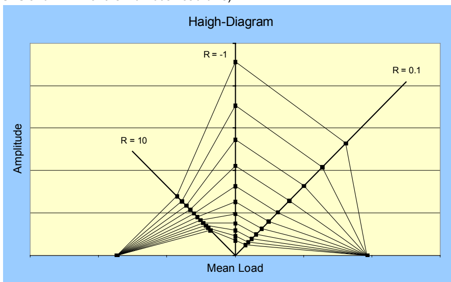
Fig. 8: Constant Life Diagram (Material data: S-N-Curves for R=-1, R=0.1, R=10, UTS,UCS - Linear interpolation between UCS/UTS and S-N-Curves for the individual load bins)
