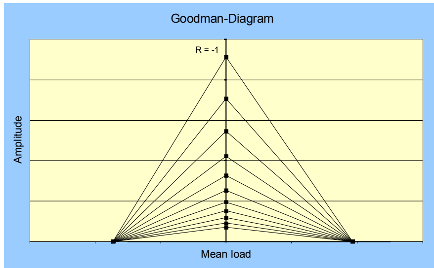
Fig. 7: Linear Goodman Diagram (Material data: S-N-Curves for R=-1, UTS,UCS - Linear interpolation between UCS/UTS and R= -1 for the individual load bins)
