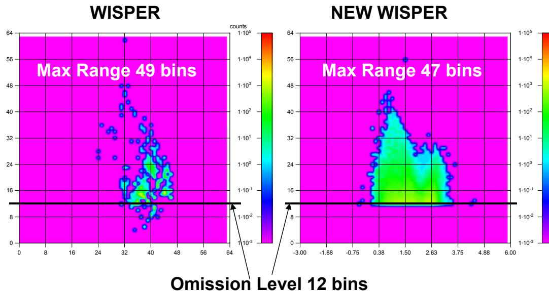
Fig.4 WISPER and NEW WISPER Range Mean Matrices
