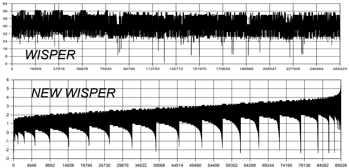
Fig.5 WISPER and NEW WISPER Sequences
